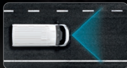
LANE CENTERING
